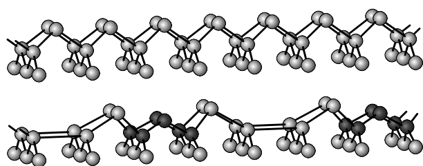
Figure 2. Scheme of the atomic arrangement of Si (light grey) and C (dark grey) along [110] . Carbon forms a complex of six atoms in between two Si dimers in each c(4 \times 4) surface unit cell. Every third dimer is missing. The paired dimers correspond to the pairs of bright spots in the STM image.
