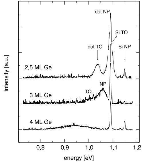
Figure 6. 4 K PL spectra of C-induced Ge dot structures on Si(001) grown at 550 °C. The C pre-deposition is kept at 0.11 ML and the Ge thickness is varied between 2.5 ML and 4 ML.
