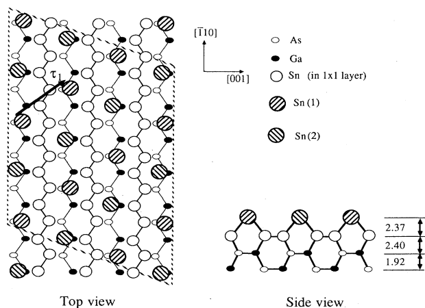
FIG. 2. Top view and side view of the proposed double-layer structure which is composed of a 1×1 Sn layer with a Sn adatom layer on top in a nominal (3×3) periodicity. The height (in Å) of the different Sn layers with respect to the GaAs substrate is indicated in the side view.
