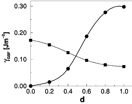
FIG. 2. Generalized stacking fault energy \gamma_{\text{GSF}} for Al with H impurities at zero tension opening, h=0 , as a function of the slip d in the [211] direction for the 1 \times 1 supercell, corresponding to H concentration of 14.3 at. %: circles represent the energy for the tetrahedral site, squares for the octahedral site (lines are fits intended as guide to the eye).
