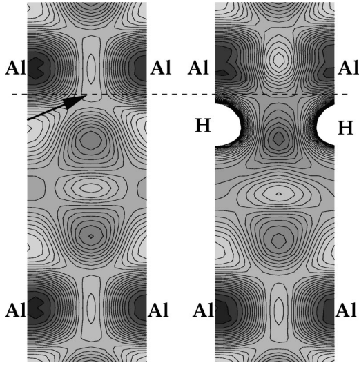
FIG. 3. Bonding valence charge density on the (\bar{1}21) plane for pure Al (left) and Al+H (right) systems at d=0 . The horizontal direction is [10\bar{1}] and the vertical direction is [111] . The fictitious slip plane is shown as a dashed line and the positions of atoms are indicated by the corresponding labels. The arrow indicates the buildup of valence charge density corresponding to covalent bonding across the slip plane.
