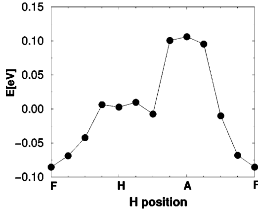
FIG. 5. Adsorption energy for H on the (111) Al surface within the 1 \times 1 surface unit cell corresponding to H coverage \Theta = 1 ML, for different positions in the [211] direction: F = fcc site, H = hcp site, A = atop site.
